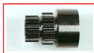
Campane cambio Gearbox clutch bells Kupplungsglocken Cloche boîte de vitesse Art. 755080000 Z 15-18 Art. 755090000 Z 15-19 Art. 755100000 Z 16-19 Art. 755110000 Z 16-20 Art. 755120000 Z 17-20 Art. 755130000 Z 17-21
