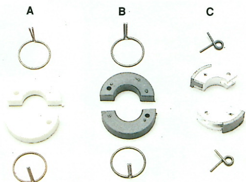
Gruppi frizioni - Clutch set A = Art. 20290 EXPERT Teflon B = Art. 20300 BUGGY Carbon C = Art. 20301 PRO Ergal-Carbon
